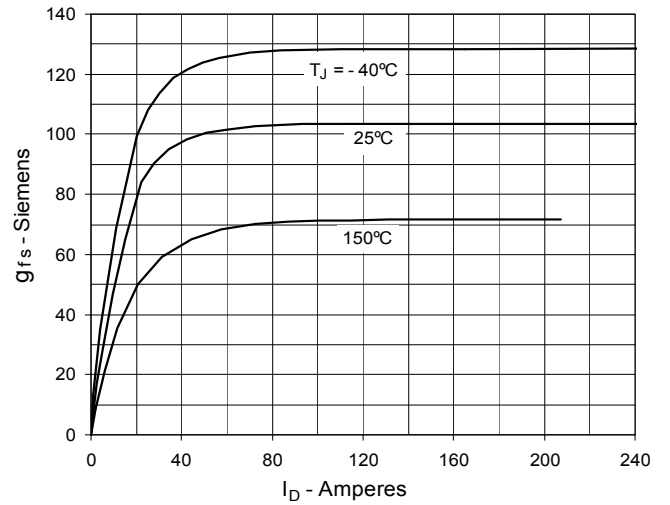
Fig. 8. Transconductance
